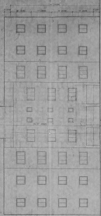
BLOCK 4 ELEVATION A (EASTERN ELEVATION)
